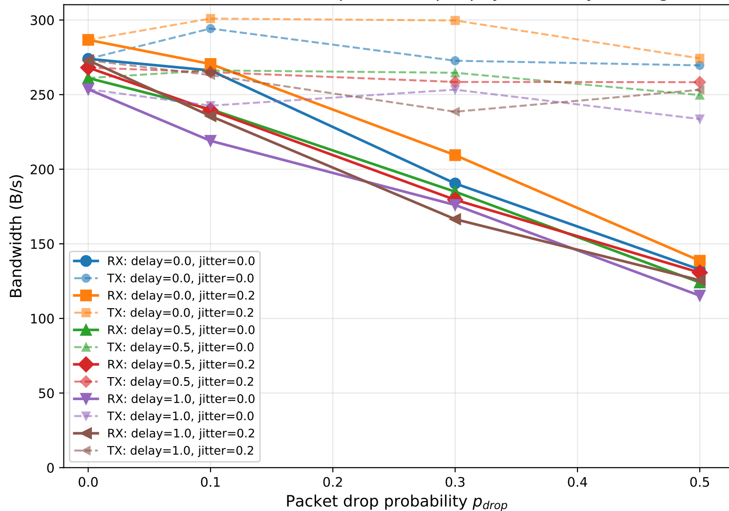
Delivered bandwidth vs packet drops (payload=6 bytes/msg)
